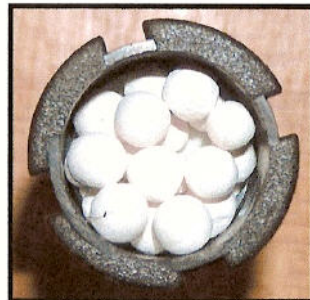
4. Fill with the alumina balls
